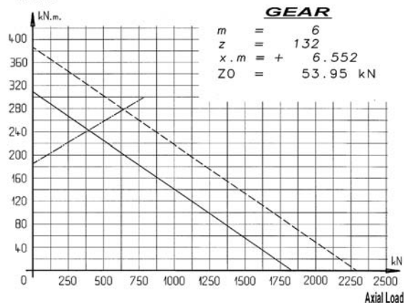
Tilting Moment
