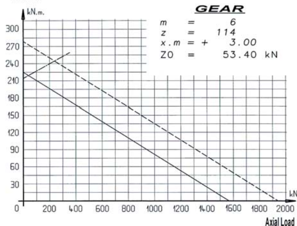
Tilting Moment
