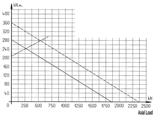
Tilting Moment
