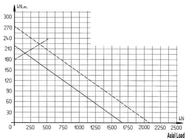
Tilting Moment
