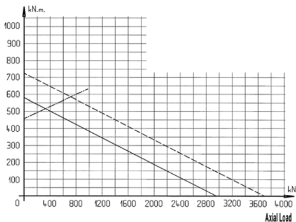
Tilting Moment
